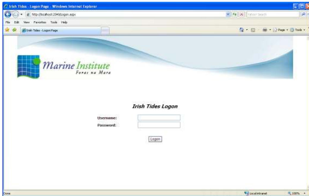
Figure 10 Logon Page
